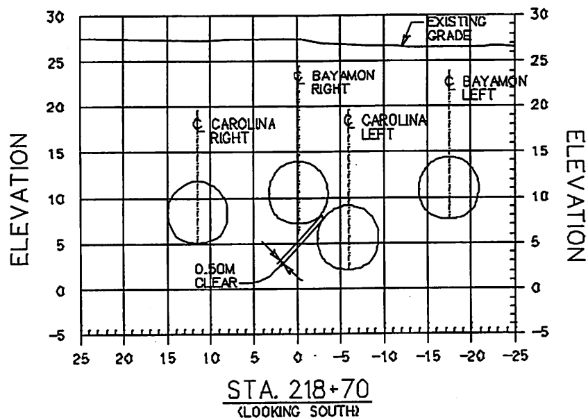
Figure 8. Mined Tunnels Cross-Section at Station 218+70
