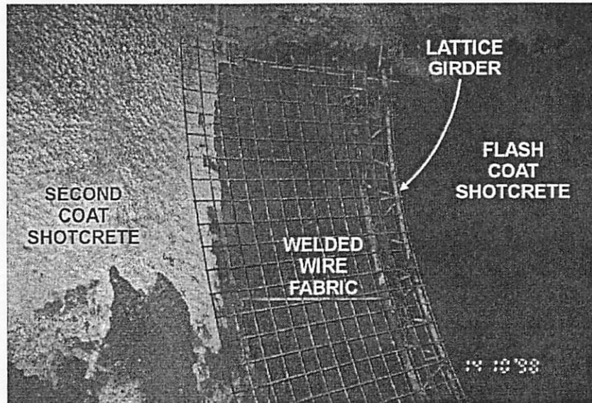
Figure 9. Lattice Girder and Mesh Reinforced Shotcrete Lining
