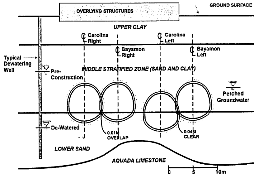
Figure 5. Typical Geotechnical Profile for Mined Tunnels
