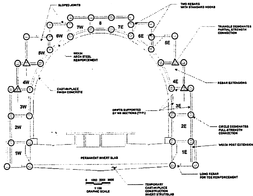
Figure 11. Structural Requirements for Stacked Drift Tunnel Reinforcement
