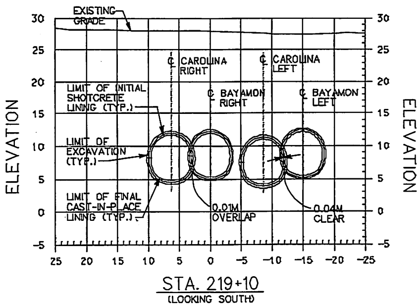
Figure 7. Mined Tunnels Cross-Section at Station 219+10
